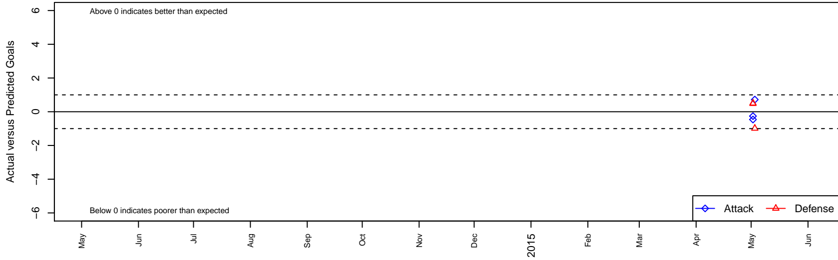
Green River Spurs G99 Dots are actual minus expected GF (blue circles) and GA (red triangles). Blue line is smoothed change in attack strength. Red is smoothed change in defense strength.
